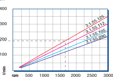
PORTATA / CAPACITY
